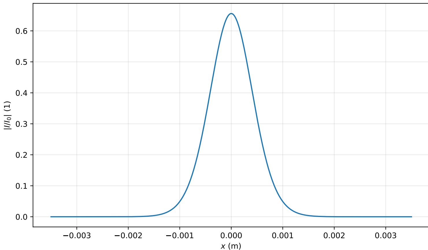
Intensity profile I(x, y = 0, z = 1.990m)/I_0 , P_{in}=0.3P_{cr} , artificial time
